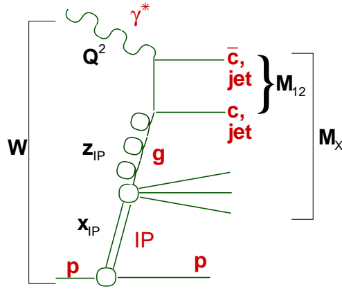
Figure 2: Diagram for jet or heavy quark pair production in the diffractive scattering of a virtual photon ( \gamma^* ), emitted by the beam electron, off the proton ( p ).
