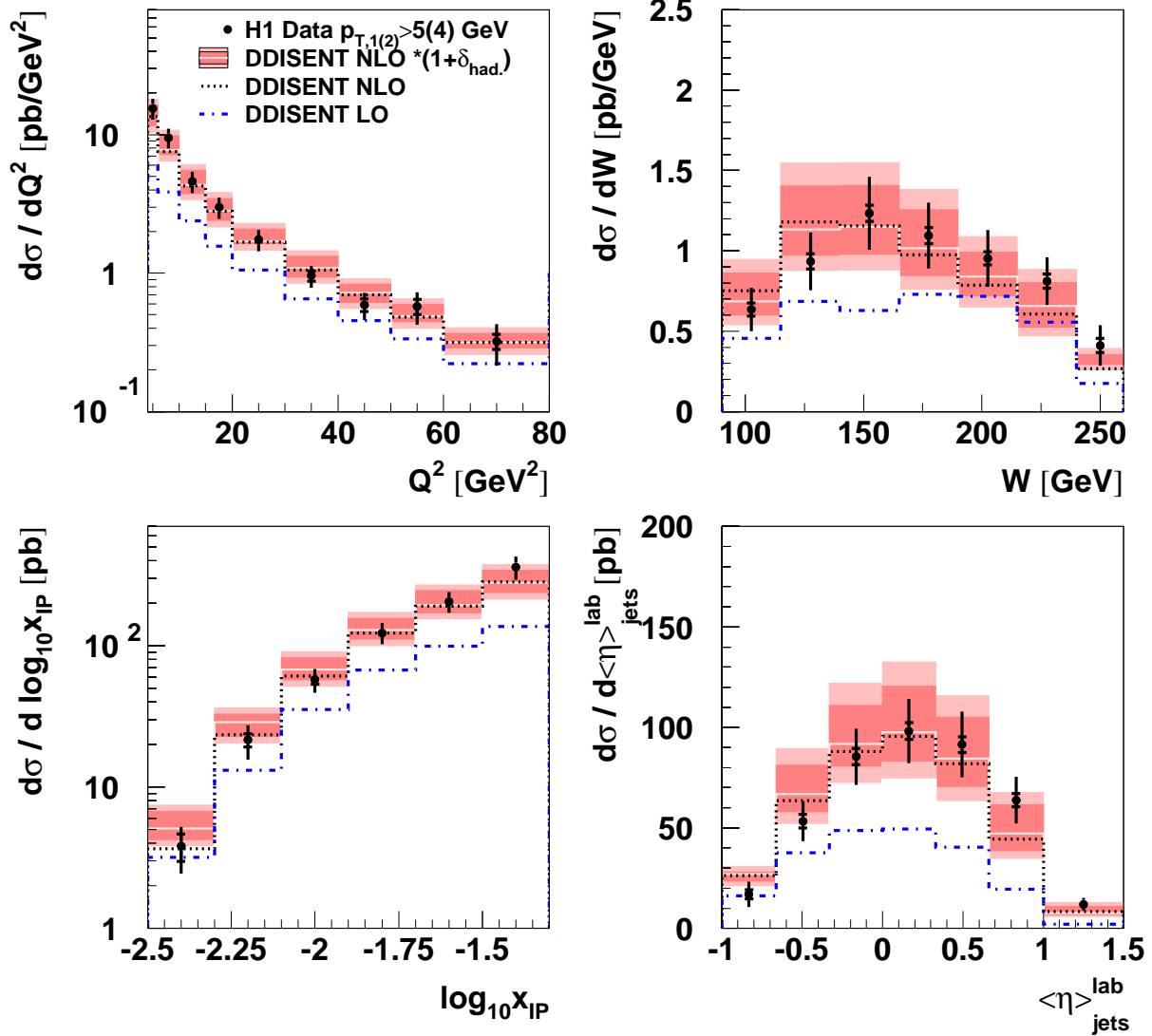
Figure 5: Differential cross section for dijet production in diffractive DIS from [7] (points), corrected to asymmetric cuts on the jet transverse momentum p_{T,1(2)}^* > 5(4) \text{ GeV} , shown as a function of the photon virtuality Q^2 , the photon-proton centre-of-mass energy W , the longitudinal proton momentum fraction taken by the diffractive exchange x_{IP} and the average pseudorapidity of the jets \langle \eta \rangle_{jets}^{lab} . The data are compared with predictions based on the (N)LO diffractive parton distributions from [3], using \mu_r^2 = p_T^2 and \mu_f^2 = 40 \text{ GeV}^2 . Shown are predictions obtained with DISSENT (using the x_{IP} slicing technique, see text) at leading order QCD (blue, dash-dotted line), at next-to-leading order QCD (black, dotted line) and at next-to-leading order including hadronization corrections (central line of error band). The inner error band represents the renormalization scale uncertainty, while the outer band also includes the uncertainty in the hadronization corrections, added linearly.
