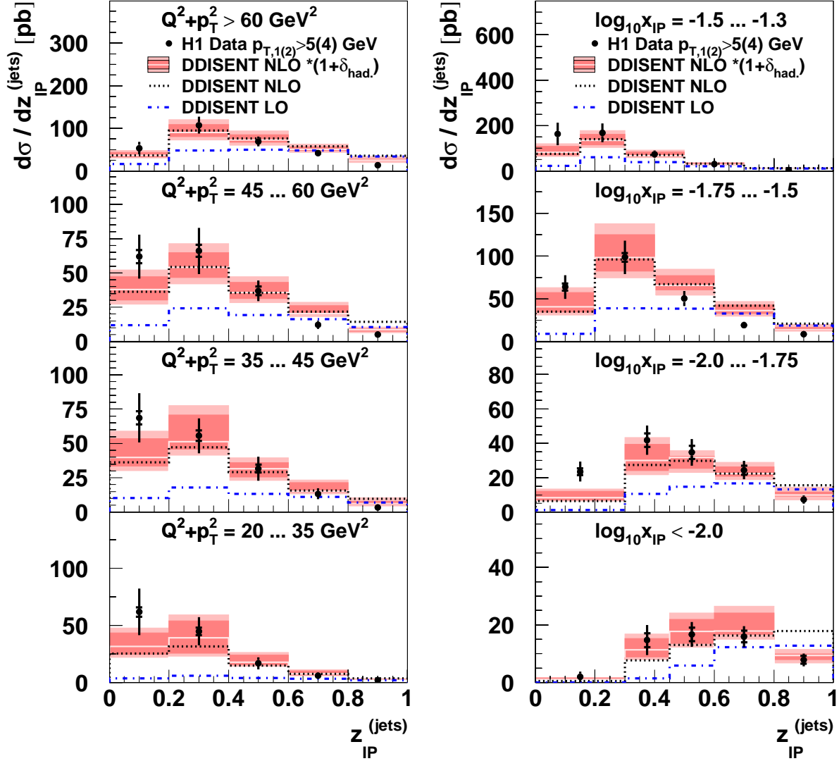
Figure 4: Differential cross section for dijet production in diffractive DIS from [7] (points), corrected to asymmetric cuts on the jet transverse momentum p_{T,1(2)}^* > 5(4) \text{ GeV} , shown as a function of z_{IP}^{(jets)} , an estimator for the momentum fraction of the longitudinal momentum fraction of the diffractive exchange entering the hard process, for four intervals of Q^2 + p_T^2 (left) and x_{IP} (right), respectively. The data are compared with predictions based on the (N)LO diffractive parton distributions from [3], using \mu_r^2 = p_T^2 and \mu_f^2 = 40 \text{ GeV}^2 . Shown are predictions obtained with DISSENT (using the x_{IP} slicing technique, see text) at leading order QCD (blue, dash-dotted line), at next-to-leading order QCD (black, dotted line) and at next-to-leading order including hadronization corrections (central line of error band). The inner error band represents the renormalization scale uncertainty, while the outer band also includes the uncertainty in the hadronization corrections, added linearly.
