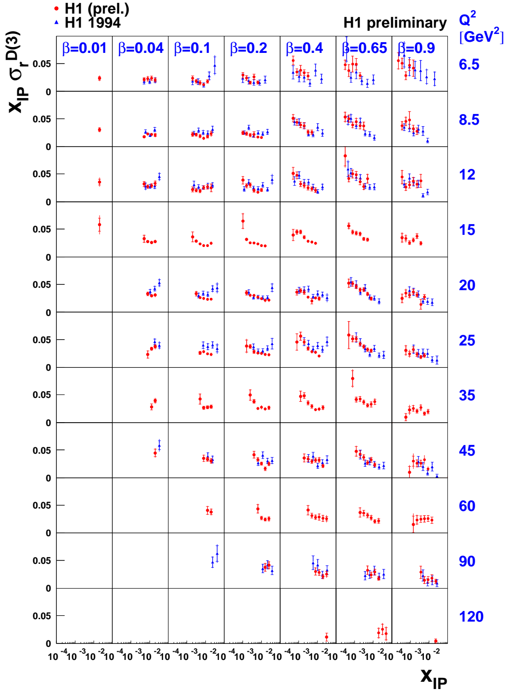
Figure 2: The measured diffractive reduced cross section ( filled circles ), presented as x_{IP}\sigma_r^{D(3)} and plotted as a function of x_{IP} at fixed values of \beta and Q^2 . Here and in all other figures, the inner error bars correspond to the statistical error, the outer error bars show the statistical and the systematic error added in quadrature. An additional normalisation uncertainty of 6.7% is not shown. For comparison, the previous H1 measurement in [3] is also shown ( triangles ).
