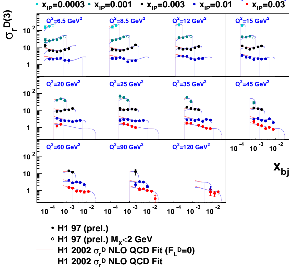
Figure A5: x dependence of the reduced cross section at fixed x_{IP} = 0.0003, 0.001, 0.003, 0.01, 0.03 and fixed Q^2 , compared with the predictions of the NLO QCD fit.
