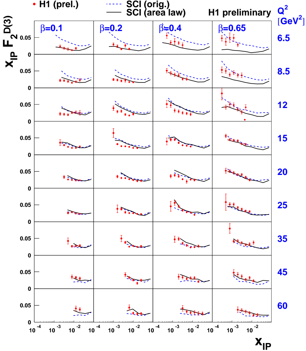
Figure 9: The diffractive structure function x_{\mathcal{P}} F_2^{D(3)}(\beta, Q^2, x_{\mathcal{P}}) , extracted from the measured reduced cross section \sigma_r^{D(3)} under the assumption of F_L^D = 0 , plotted as a function of x_{\mathcal{P}} at fixed values of Q^2 and \beta . Only a sub-sample of the data, corresponding to 0.1 \leq \beta \leq 0.65 and Q^2 \leq 60 \text{ GeV}^2 , are shown. The data are compared with the predictions of the original Soft Colour Interactions (SCI) model [35] ( dashed curves ) and its refinement based on a generalised area law [36] ( solid curves ). The predictions have been obtained using the LEPTO 6.5.2 \beta Monte Carlo generator [37].
