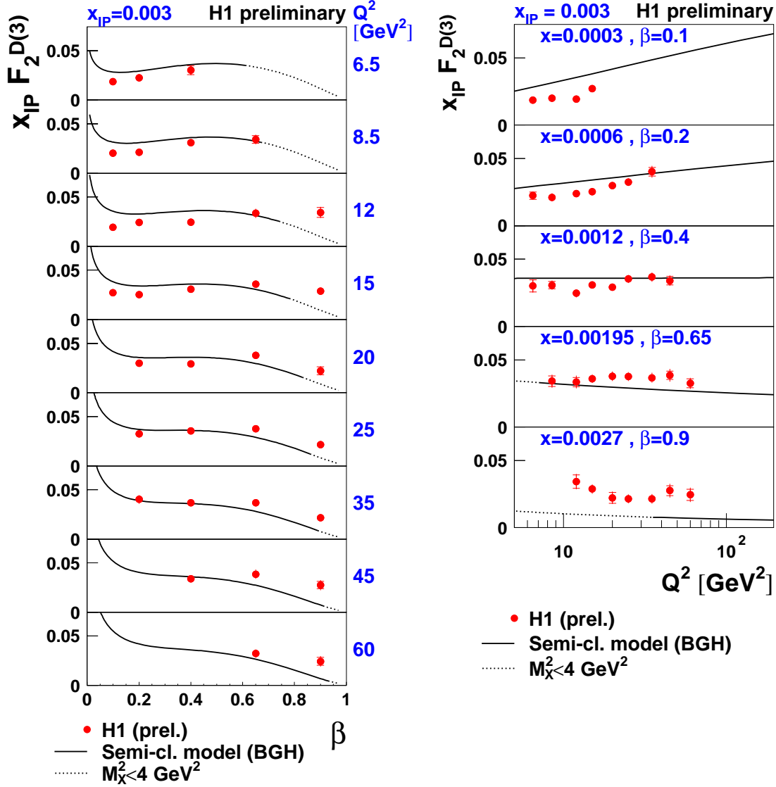
Figure 7: The diffractive structure function x_{IP} F_2^{D(3)}(\beta, Q^2, x_{IP}) , extracted from the measured reduced cross section \sigma_r^{D(3)} under the assumption of F_L^D = 0 , at fixed x_{IP} = 0.003 , plotted as a function of \beta for various values of Q^2 (left) and as a function of Q^2 for various values of \beta (right). The data are compared with the predictions of the semi-classical model by Buchmüller, Gehrman and Hebecker [32] (solid curves). The dotted curves correspond to an extension of the model into the region of small M_X < 2 \text{ GeV} , where the model is not expected to be valid.
