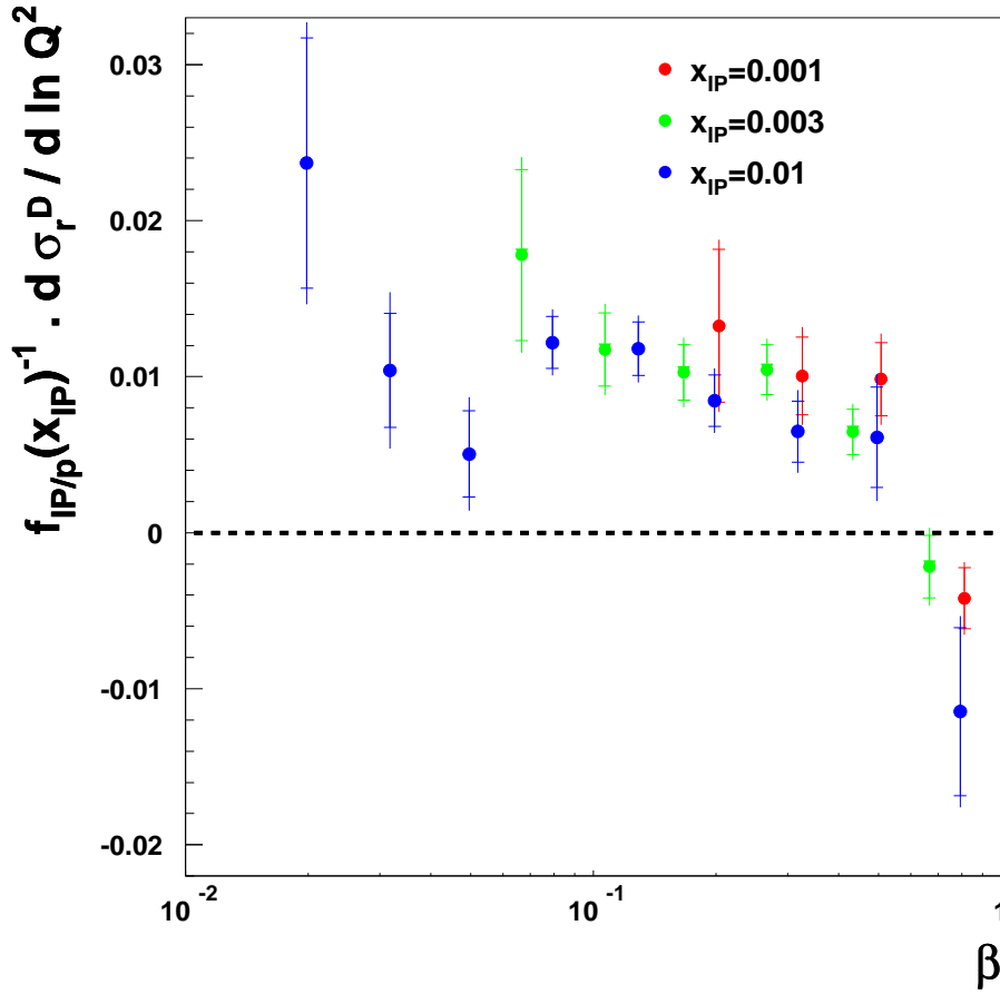
Figure 6: Logarithmic Q^2 derivatives of \sigma_r^D for different \beta and x_{IP} = 0.001, 0.003, 0.01 , scaled at each x_{IP} by the values assumed for the t -integrated pomeron flux in the QCD fits (equation 14).
