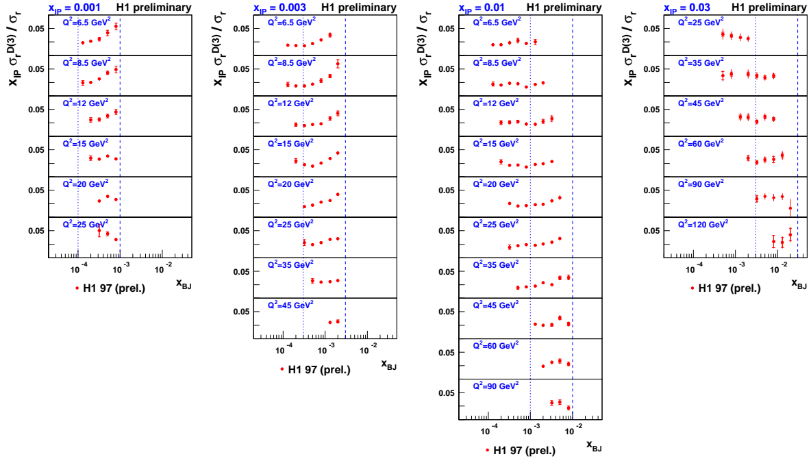
Figure 12: The ratio of diffractive to inclusive reduced cross sections, shown as a function of x at fixed x_P and Q^2 values. Note that M_x^2 = Q^2(x_P/x - 1) varies with x in these plots. The dashed (dotted) lines indicate the points at which \beta = 1 ( \beta = 0.1 ). Clear variations in the shape are observed for the different x_P values, arising from the fact that they cover different \beta ranges. For the high \beta region, the ratio has a complicated shape, since \sigma_r^D has considerable structure in this region, whereas \sigma_r is well parameterised by x^{-\lambda} . For the lowest \beta , a flatter dependence of the ratio on x is observed.
