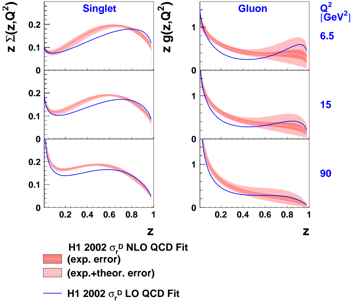
Figure 14: Diffractive parton densities obtained from the QCD fit, normalised such that the ‘pomeron flux’ is unity at x_{\mathbb{P}} = 0.003 . The left hand side shows the singlet quark distribution ( 6 * u where we assume u = d = s = \bar{u} = \bar{d} = \bar{s} ). The right hand side shows the gluon density. The red bands show the results of the NLO fits, with inner error bands showing the experimental errors (statistical and systematic) and the outer error bands showing the full uncertainties, including those arising from theoretical assumptions. For comparison, the central values of the parton densities extracted from the LO fit are also shown (blue line).
