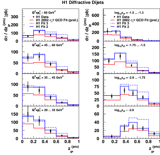
Figure A10: H1 measurements [11] of diffractive dijet cross sections as a function of z_{IP}^{\text{jets}} in different intervals of Q^2 + p_{T,\text{jets}}^{*2} (left) and of x_{IP} (right), compared with the new and old [3] LO QCD fits.
