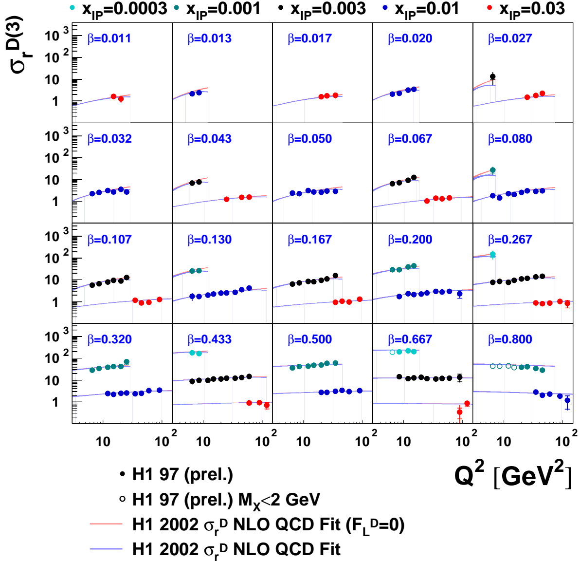
Figure A4: Q^2 dependence of the reduced cross section at fixed x_{IP} = 0.0003, 0.001, 0.003, 0.01, 0.03 and fixed \beta or x , compared with the predictions of the NLO QCD fit. The filled data points were included in the fit. The open data points ( M_x < 2 GeV) were omitted. The predictions of the NLO fit for F_2^D (i.e. \sigma_r^D for F_L^D = 0 ) are also shown.
