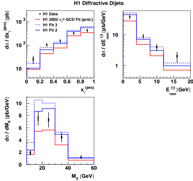
Figure A11: H1 measurements [11] of diffractive dijet cross sections differential in the fraction x_{\gamma}^{\text{jets}} of the virtual photon momentum transferred to the dijet system, the energy E_{\text{rem}}^{\gamma} in the photon hemisphere reconstructed outside the jets and M_X , compared with the new and old [3] LO QCD fits.
