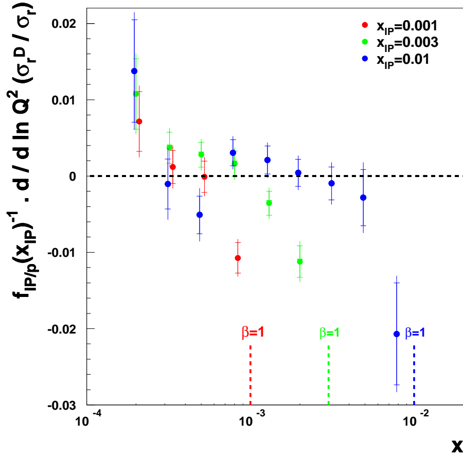
Figure 11: Logarithmic Q^2 derivatives of the ratio \sigma_r^D/\sigma_r , the x_{IP} dependence of \sigma_r^D having been divided out using a parameterisation of the x_{IP} dependence (equation 14). The data are consistent with identical Q^2 dependences of the diffractive and inclusive cross sections away from \beta = 1 , with clear differences from this behaviour as \beta \rightarrow 1 .
