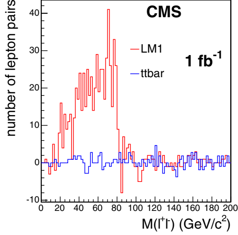
Figure 13.9. Invariant mass distribution of \mu^+\mu^- + e^+e^- and \mu^\pm e^\mp pairs at point LM1 for 1\text{ fb}^{-1} luminosity after subtracting e^+\mu^- and \mu^+e^- pairs. The contribution from the t\bar{t} background is also shown.
