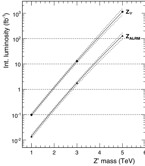
Figure 3.21. Integrated luminosity needed to reach 5\sigma significance ( S_L = 5 ) as a function of Z' mass for Z_\psi and Z_{\text{ALRM}} models. Solid lines show the best estimates, dashed lines indicate boundaries of the band corresponding to the predictions with \pm 1\sigma theoretical uncertainty.
