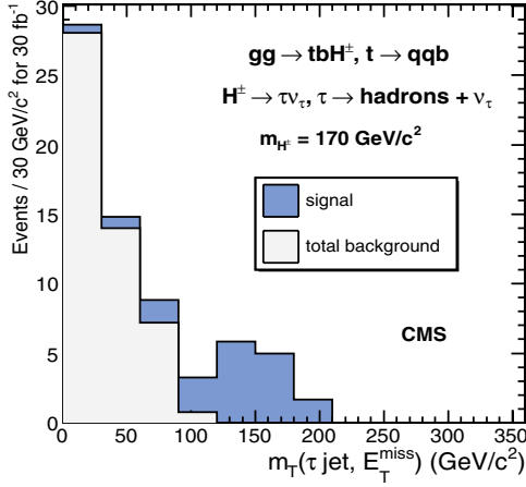
Figure 11.17. Transverse mass reconstructed from the \tau jet and missing transverse energy for the gg \rightarrow tbH^\pm , t \rightarrow qqb , H^\pm \rightarrow \tau\nu_\tau , \tau \rightarrow \text{hadrons} + \nu_\tau with m_{H^\pm} = 170 \text{ GeV}/c^2 , \tan\beta = 30 and for the total background (light histogram) for an integrated luminosity of 30 \text{ fb}^{-1} .
