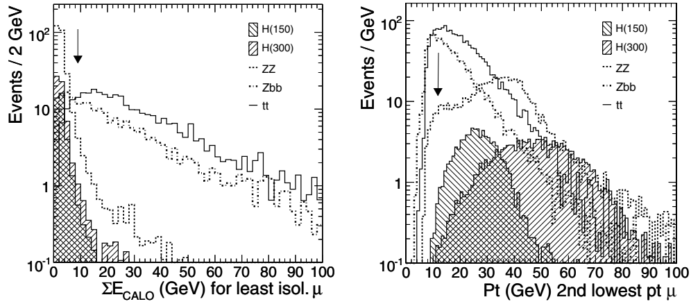
Figure 3.3. Examples of discriminating variables: (left) muon calorimeter-based isolation \sum E_T for the least isolated muon and (right) transverse momentum of the 2 nd lowest p_T muon. The hatched histograms represent the Higgs boson signals of masses 150 GeV/ c^2 and 300 GeV/ c^2 , while the solid, dashed and dash-dotted lines indicate the contribution from the t\bar{t} , ZZ and Zbb backgrounds, respectively. The arrows indicate the positions of the cuts.
