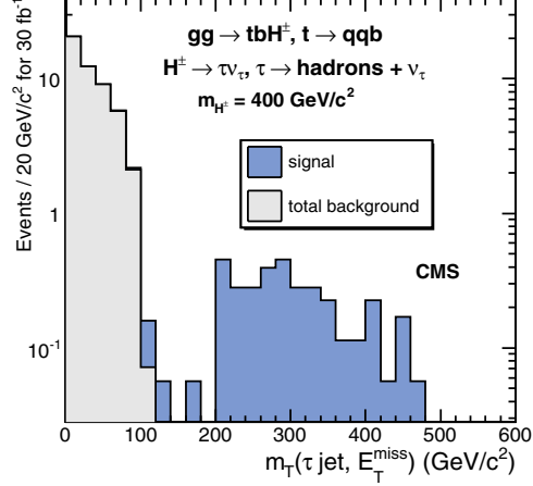
Figure 11.18. Transverse mass reconstructed from the \tau jet and missing transverse energy for the gg \rightarrow tbH^\pm , t \rightarrow qqb , H^\pm \rightarrow \tau\nu_\tau , \tau \rightarrow \text{hadrons} + \nu_\tau with m_{H^\pm} = 400 \text{ GeV}/c^2 , \tan\beta = 30 and for the total background (light histogram) for an integrated luminosity of 30 \text{ fb}^{-1} .
