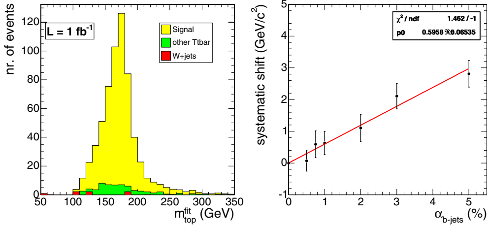
Figure 8.6. Left: Distribution of the mass of the hadronic decaying top quark for the selected events after applying the kinematic fit. Right: Estimated shift in M_t^{\text{FullIdeo}} versus a relative shift \alpha applied on the inclusive heavy quark jet energy scale.
