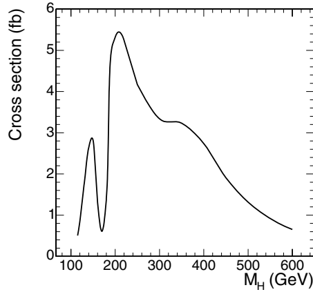
Figure 3.1. Standard Model NLO cross section for the process (ZZ^{(*)} \rightarrow 4\mu) vs. Higgs boson mass.
