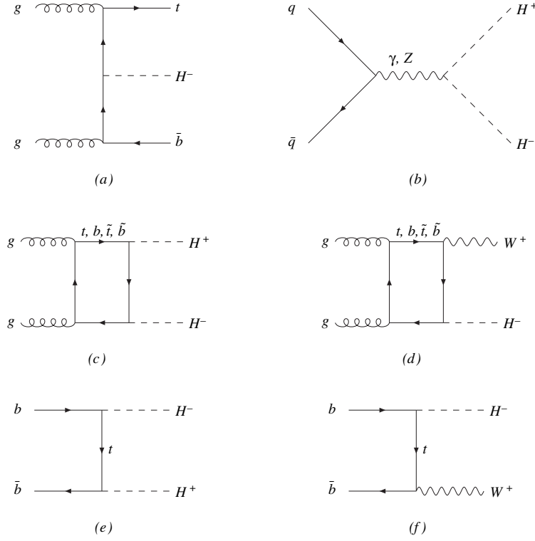
Figure 11.5. Typical diagrams for charged Higgs boson production mechanisms at leading order: (a) gg \to H^- t \bar{b} , (b) q\bar{q} \to H^+ H^- , (c) gg \to H^+ H^- , (d) gg \to W^+ H^- , (e) b\bar{b} \to H^+ H^- , (f) b\bar{b} \to W^+ H^- .
