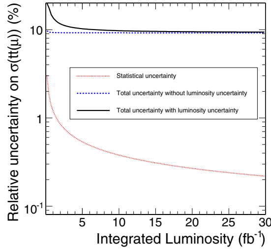
Figure 8.3. Statistical and total uncertainty on the inferred cross section of the process pp \rightarrow t\bar{t} \rightarrow bq\bar{q}b\bar{\mu}\nu_{\mu} as a function of the integrated luminosity.
