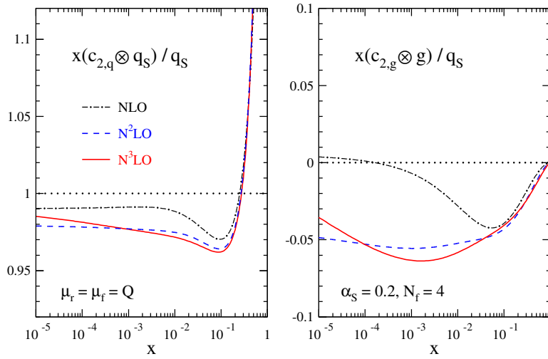
Fig. 6: The perturbative expansion up to three loops ( N^3\text{LO} ) of the quark (left) and gluon (right) contributions to singlet structure function F_2 .
