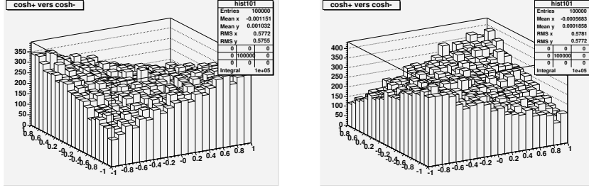
Fig. 1: The correlations between \cos \Theta (azimuthal angle) of lepton and antilepton from t\bar{t} \rightarrow \ell\nu\bar{\ell}\nu\bar{\ell}\bar{b} decays measured in the rest frame of the top-quark with respect to the anti-top quark direction. Left plot is for gg \rightarrow (WW\bar{b}\bar{b}) \rightarrow f\bar{f}f\bar{f}b\bar{b} process, right plot for q\bar{q} \rightarrow (WW\bar{b}\bar{b}) \rightarrow f\bar{f}f\bar{f}b\bar{b} process.
