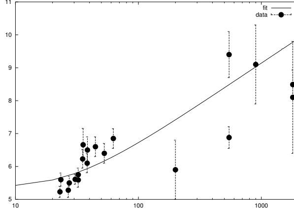
Fig. 2: Integrated SD data and a two channel model fit.
