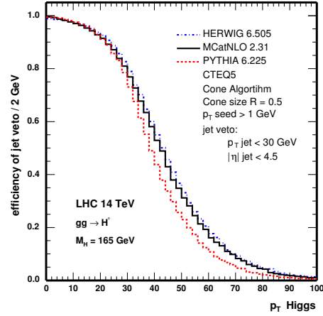
Fig. 5: Efficiency of the jet veto of 30 GeV as a function of p_T^{\text{Higgs}} .
