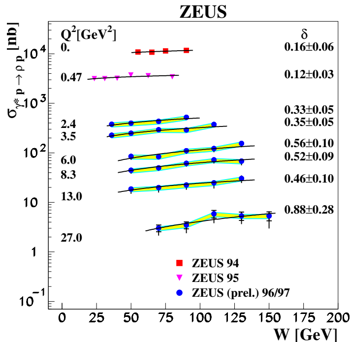
Fig. 16: Cross section for exclusive \rho production as a function of W (from [27]). The lines represent the result of fits to the data with the form \sigma(\gamma^*p \rightarrow \rho p) \propto W^\delta , yielding the exponents given in the figure.
