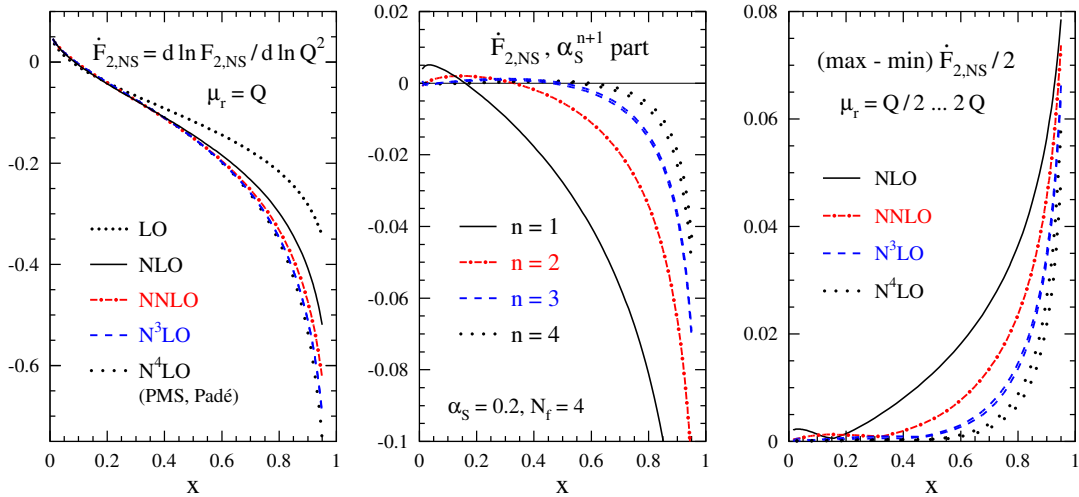
Fig. 5: The perturbative expansion of the logarithmic scale derivative of the non-singlet structure function F_{2,\text{ns}} . The results up to NNLO are exact, while those at N^3\text{LO} are very good approximations. The N^4\text{LO} corrections have been estimated by various methods.
