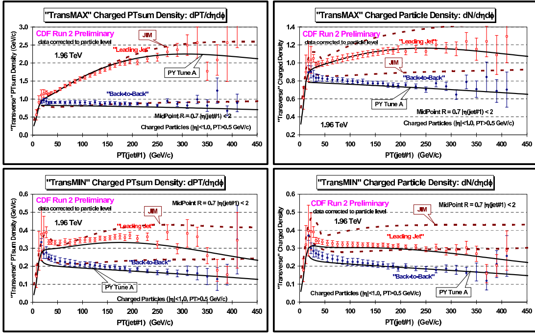
Fig. 11: Left: Data at 1.96 TeV on scalar PT sum density of charged particles, dPT_{sum}/d\phi d\eta , with p_T > 0.5 GeV/c and |\eta| < 1 in the “transMAX” region (top) and the “transMIN” region (bottom) for “leading jet” and “back-to-back” events defined in Fig. 7 as a function of the leading jet PT compared with PYTHIA Tune A and tuned JIMMY. JIMMY was tuned to fit the “transverse” energy density in “leading jet” events ( PT_{JIM} = 3.25 GeV/c). Right: Data on the density of charged particles, dN_{chg}/d\phi d\eta , with p_T > 0.5 GeV/c and |\eta| < 1 in the “transMAX” region (top) and the “transMIN” region (bottom) for “leading jet” and “back-to-back” events defined in Fig. 2 as a function of the leading jet PT compared with PYTHIA Tune A and tuned JIMMY. JIMMY was tuned to fit the “transverse” energy density in “leading jet” events ( PT_{JIM} = 3.25 GeV/c). The data are corrected to the particle level (with errors that include both the statistical error and the systematic uncertainty) and compared with the theory at the particle level (i.e., generator level).
