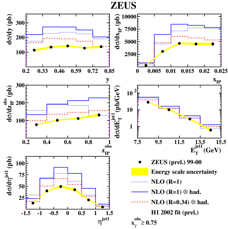
Fig. 7: Direct enriched photoproduction. Diffractive dijet photoproduction cross section differential in y , x_P , z_{IP}^{\text{jets}} , E_T^{\text{jet}1} and \eta_{\text{jet}1} compared with a NLO prediction based on diffractive PDFs. The NLO prediction is also presented corrected for hadronization effects and with the “resolved” part scaled by 0.34.
