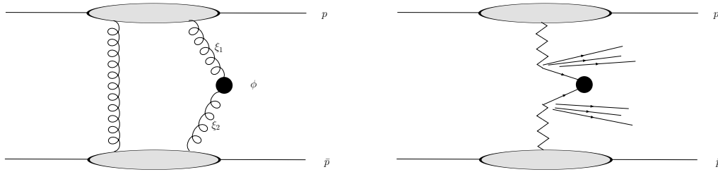
Fig. 1: The exclusive production process (a) and the inclusive (double pomeron) production process (b).
